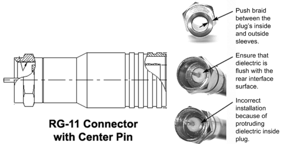
Figure 15 Attaching the RG-11 Connector
